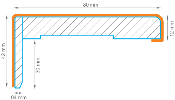
12 x 80 mm Düz Pervaz / 12 x 80 mm Straight Architrave
