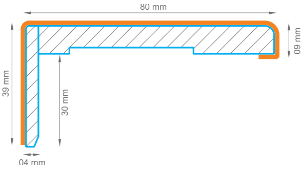
09 x 80 mm Düz Pervaz / 09 x 80 mm Straight Architrave
