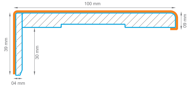
09 x 100 mm Düz Pervaz / 09 x 100 mm Straight Architrave
