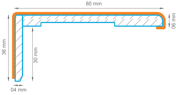
06 x 80 mm Düz Pervaz / 06 x 80 mm Straight Architrave
