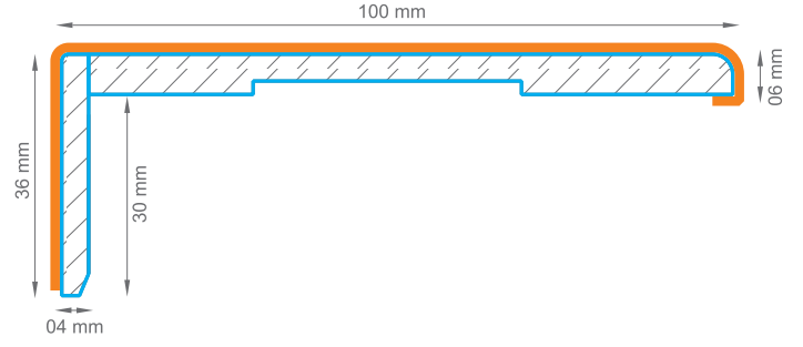
06 x 100 mm Düz Pervaz / 06 x 100 mm Straight Architrave
