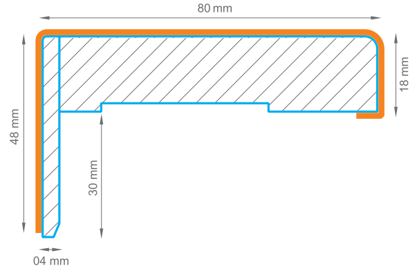
18 x 80 mm Düz Pervaz / 18 x 80 mm Straight Architrave
