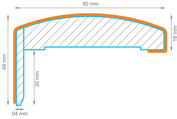
18 x 80 mm Bombeli Pervaz / 18 x 80 mm Curved Architrave
