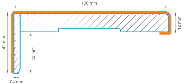
12 x 100 mm Düz Pervaz / 12 x 100 mm Straight Architrave
